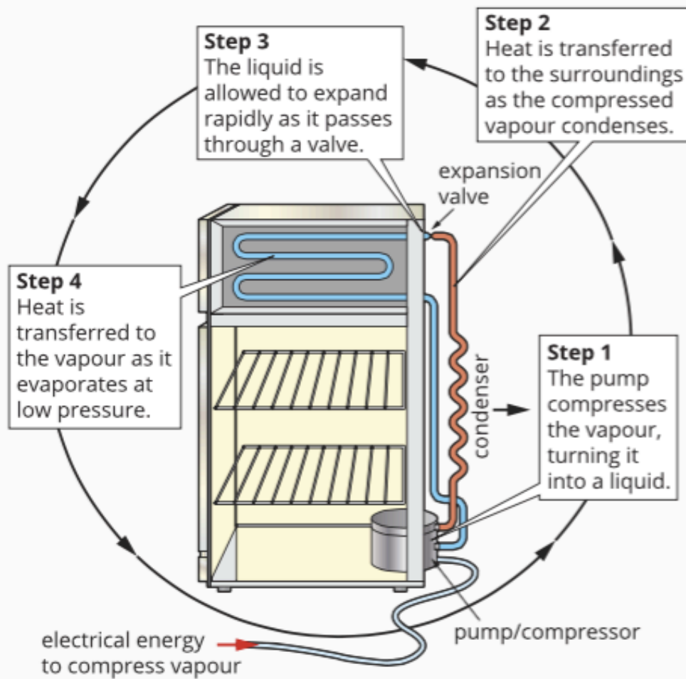
1.3.5 • A refrigerator as a heat pump to remove energy from inside the refrigerator.
